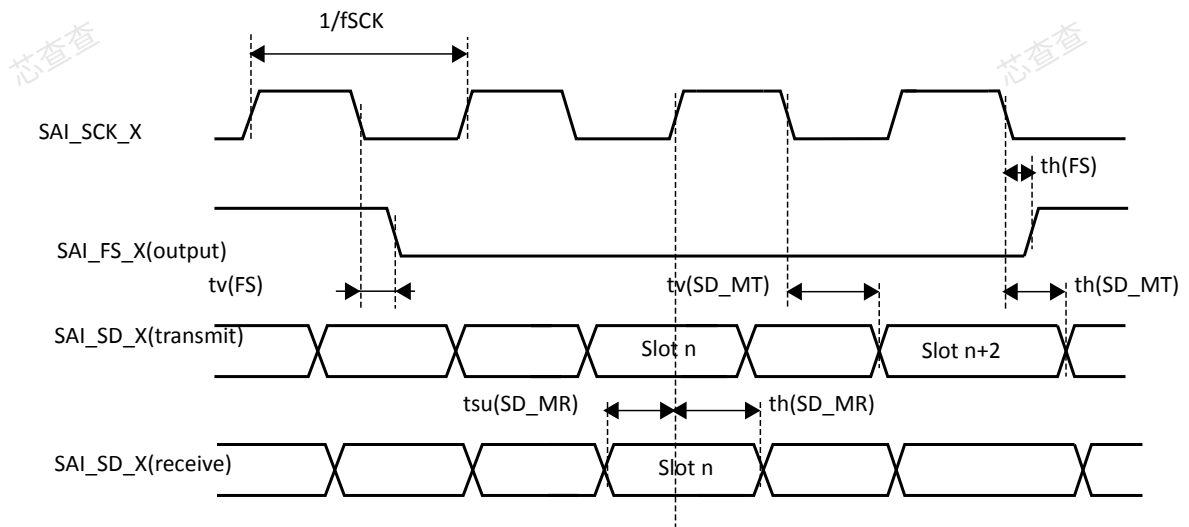
Figure 73. SAI master timing waveforms
