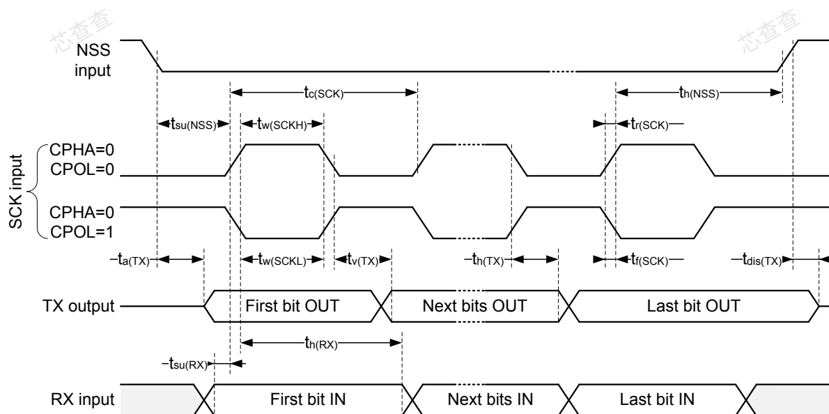
Figure 67. USART timing diagram in Slave mode
