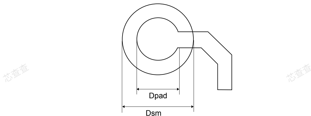
Figure 89. TFBGA100 - Recommended footprint
