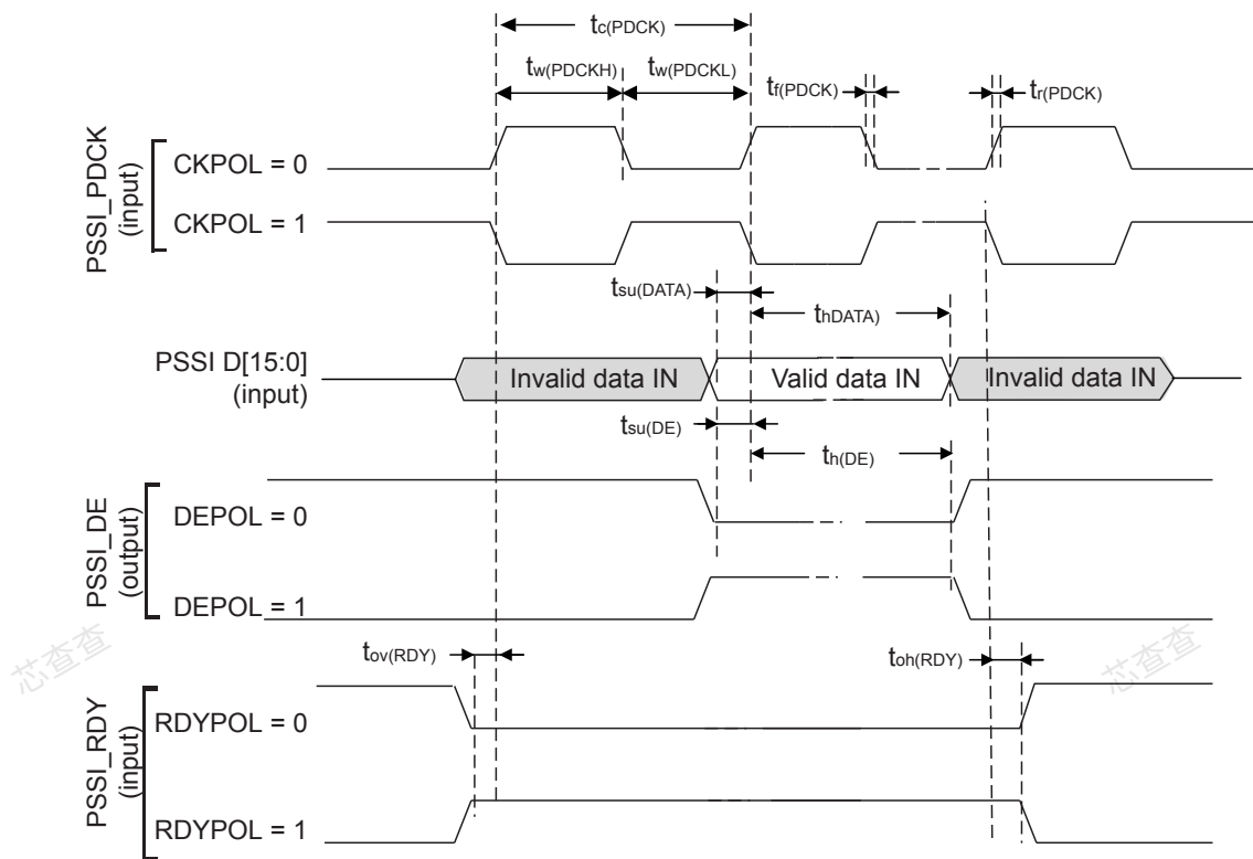
Figure 63. PSSI timing diagram in Receive mode
