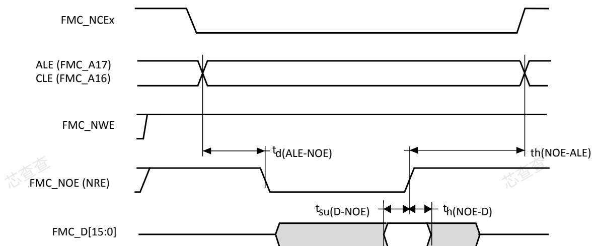
Figure 43. NAND controller waveforms for read access
