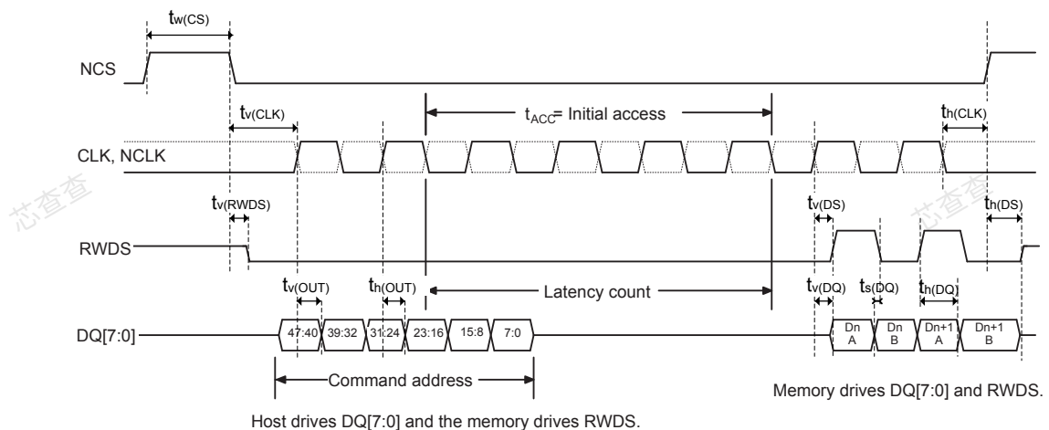
Figure 52. OctoSPI Hyperbus read
