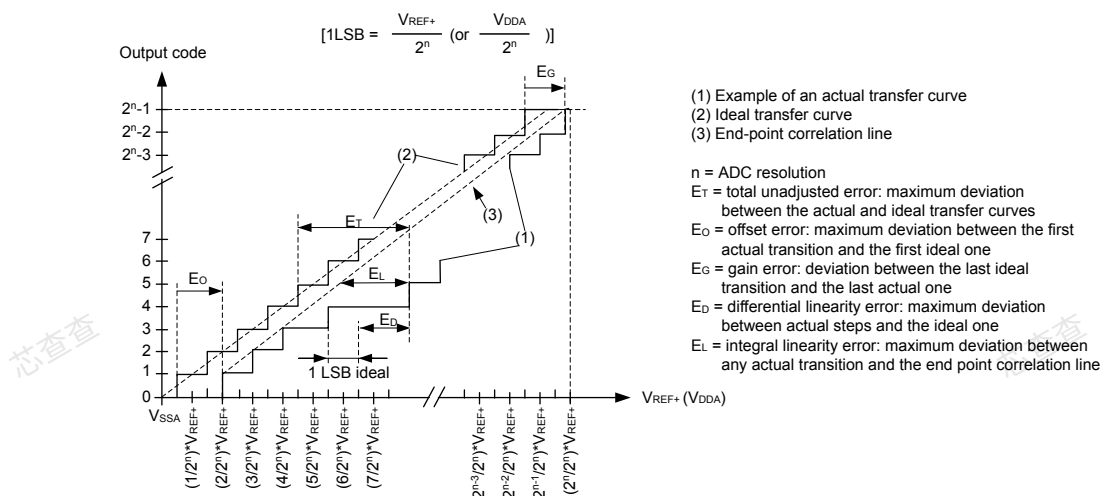
Figure 55. ADC accuracy characteristics
