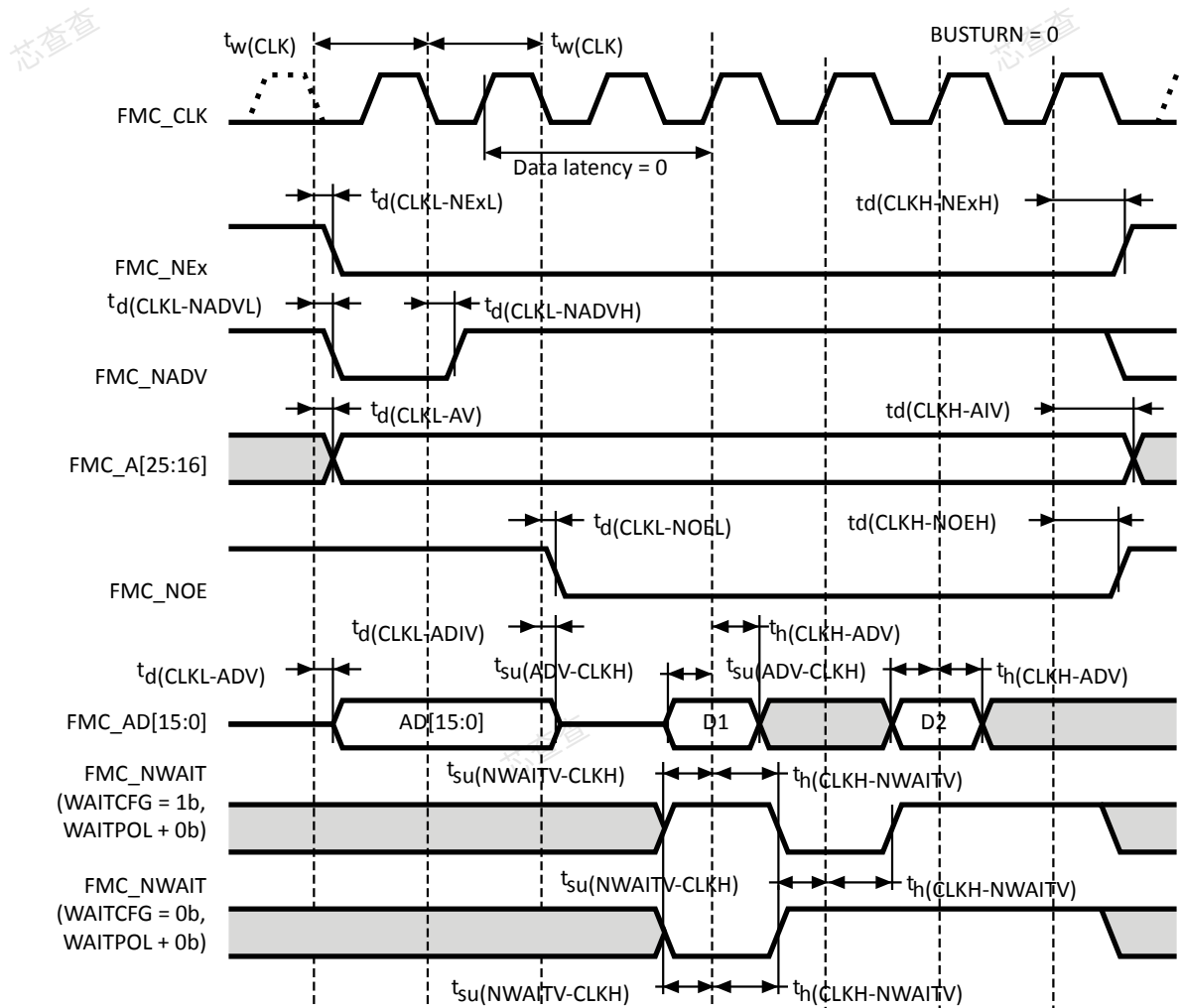
Figure 39. Synchronous multiplexed NOR/PSRAM read timings
