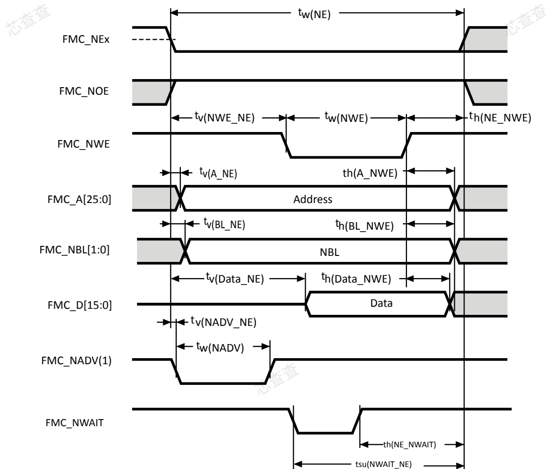
Figure 37. Asynchronous non-multiplexed SRAM/PSRAM/NOR write waveforms
