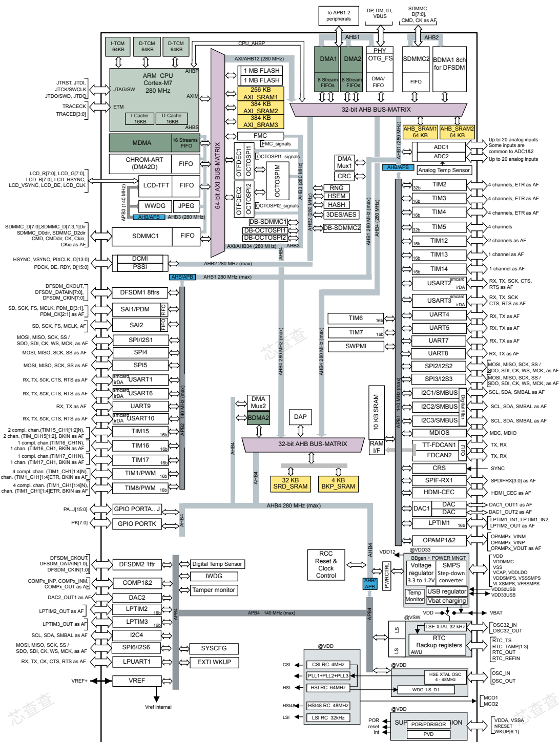
Figure 1. STM32H7B3xl block diagram
