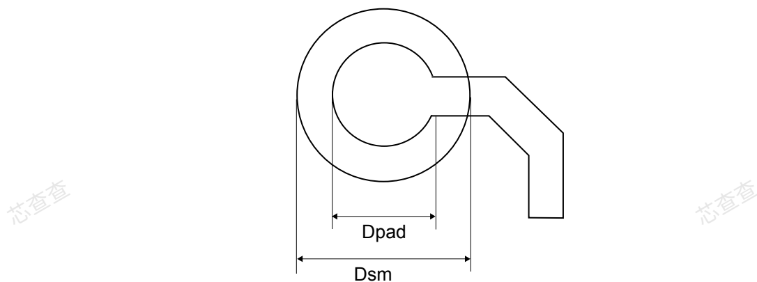
Figure 101. TFBGA216 - Recommended footprint
