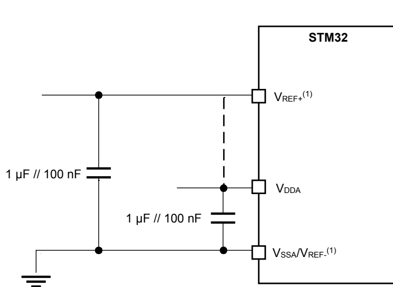
Figure 57. Power supply and reference decoupling ( V_{REF+} not connected to V_{DDA} )
