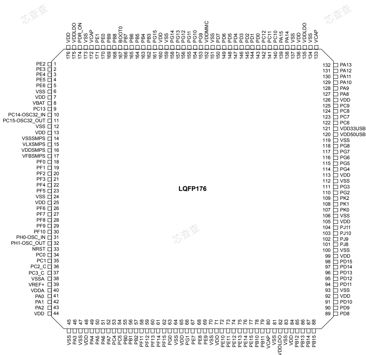
Figure 12. LQFP176 (STM32H7B3xl with SMPS) pinout
