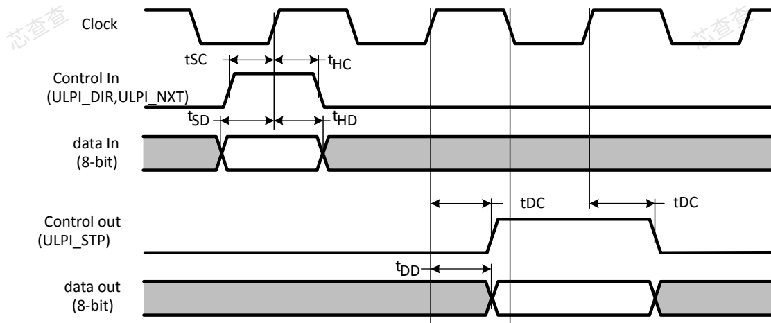
Figure 79. ULPI timing diagram
