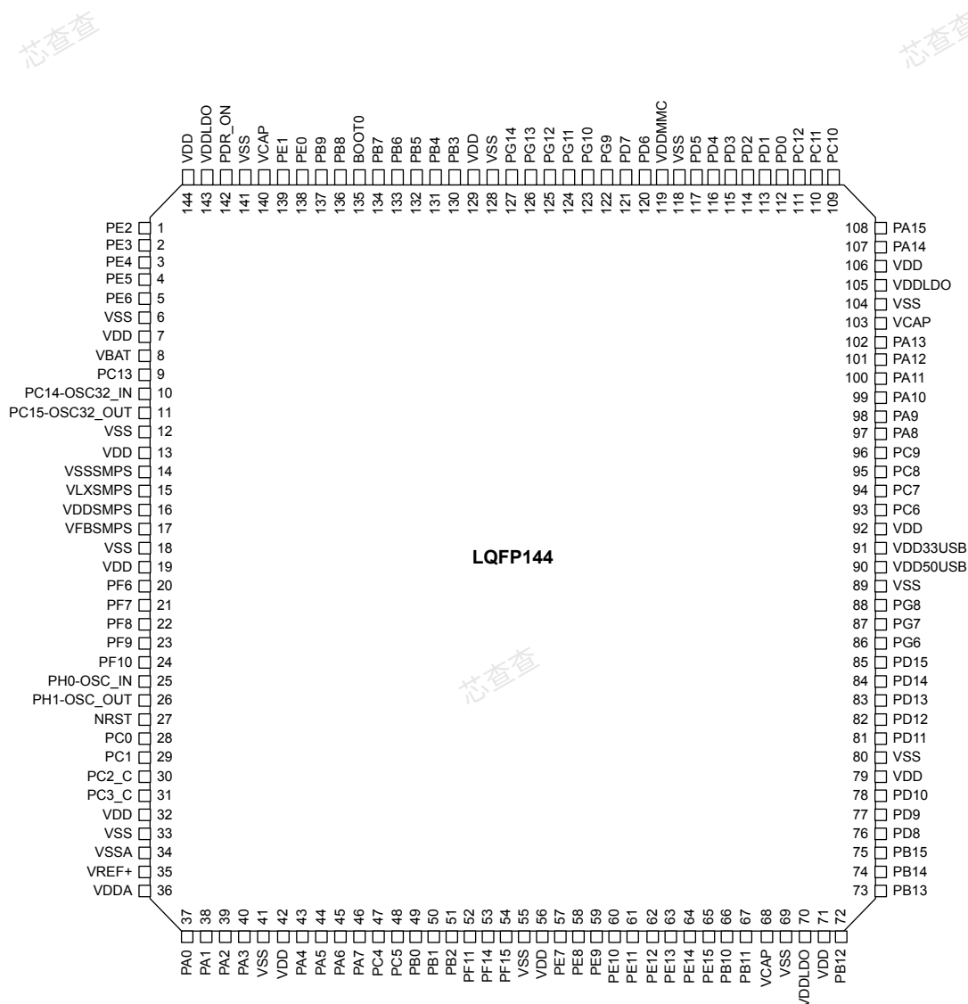
Figure 10. LQFP144 (STM32H7B3xl with SMPS) pinout
