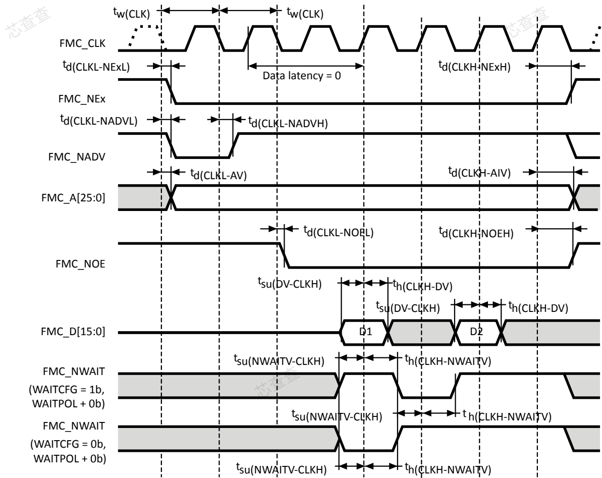
Figure 41. Synchronous non-multiplexed NOR/PSRAM read timings
