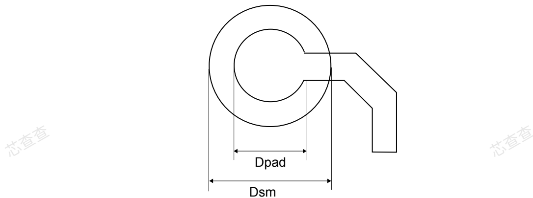
Figure 107. UFBGA169 - Recommended footprint
