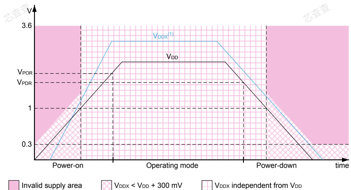
Figure 2. Power-up/power-down sequence
