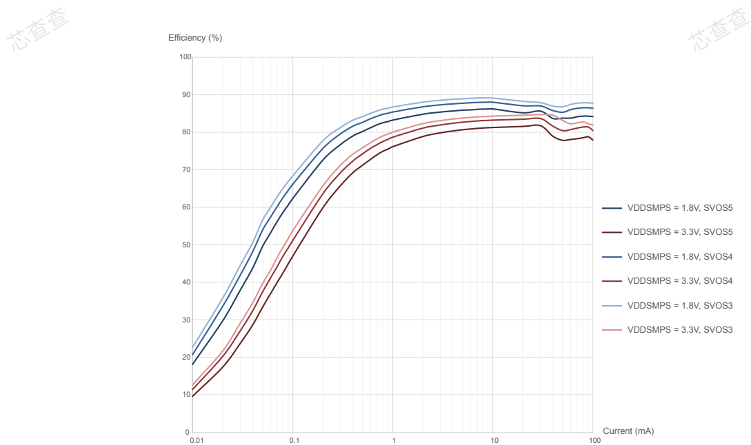
Figure 26. SMPS efficiency vs load current in Stop and DStop modes (SVOS3 LP mode, SVOS4, SVOS5), T_J = 30\text{ }^{\circ}\text{C}
