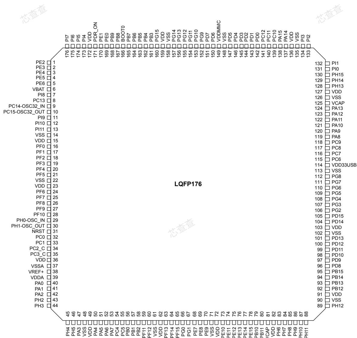
Figure 13. LQFP176 (STM32H7B3xl without SMPS) pinout
