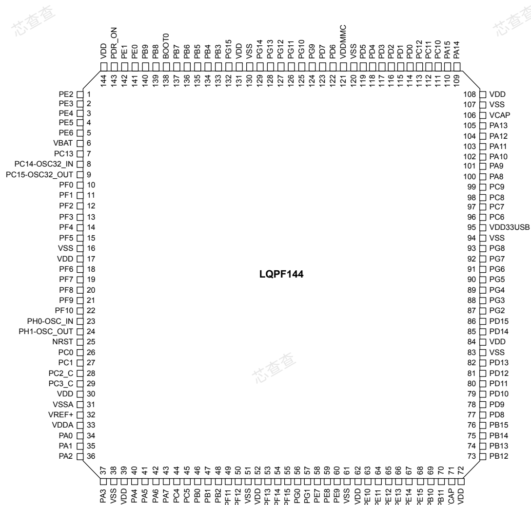
Figure 11. LQFP144 (STM32H7B3xl without SMPS) pinout
