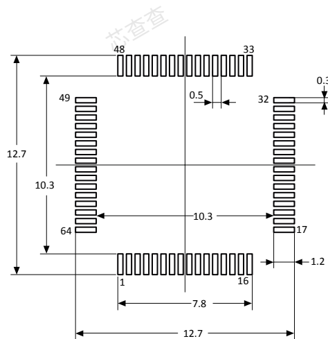
Figure 83. LQFP64 - Recommended footprint
