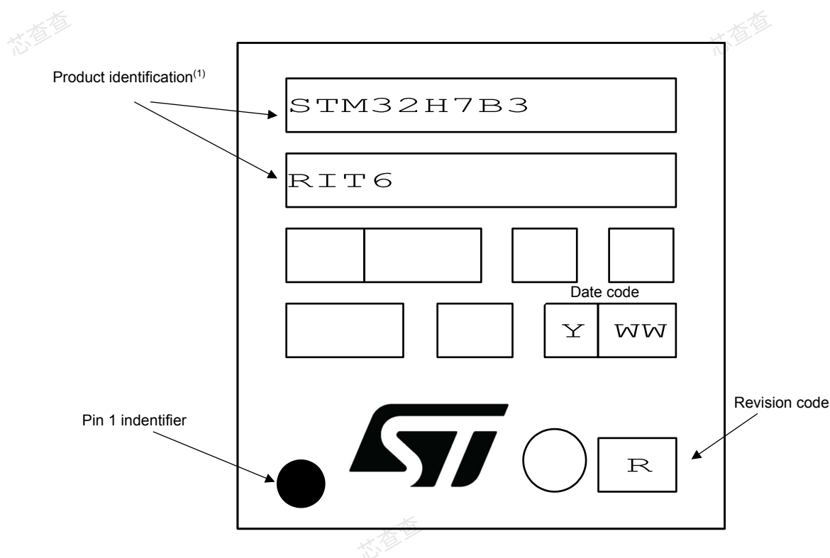
Figure 84. LQFP64 marking example (package top view)
