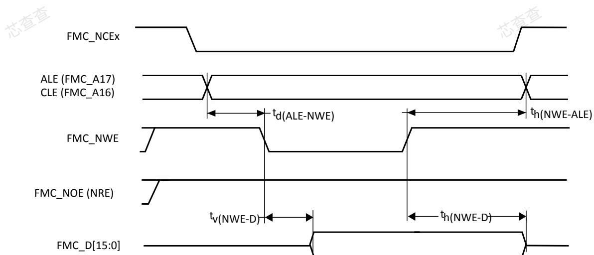
Figure 44. NAND controller waveforms for write access
