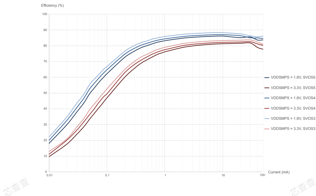
Figure 27. SMPS efficiency vs load current in Stop and DStop modes (SVOS3 LP mode, SVOS4, SVOS5), T_J = 130\text{ }^{\circ}\text{C}
