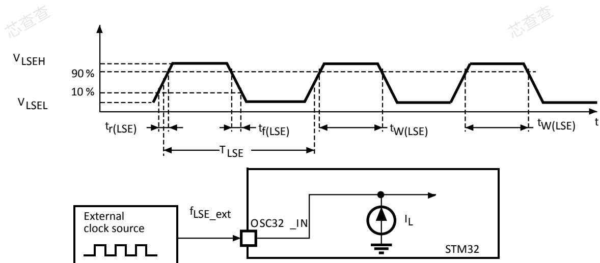
Figure 31. Low-speed external clock source AC timing diagram
