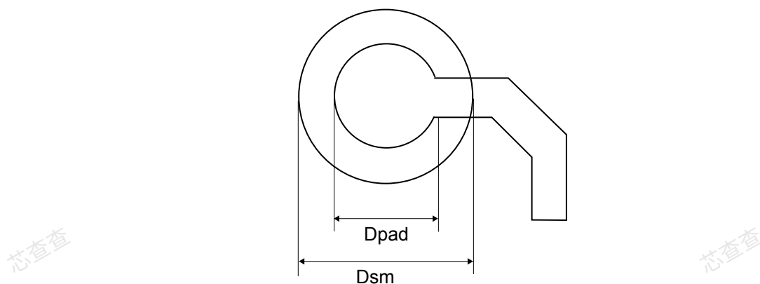
Figure 110. UFBGA(176+25) - Recommended footprint
