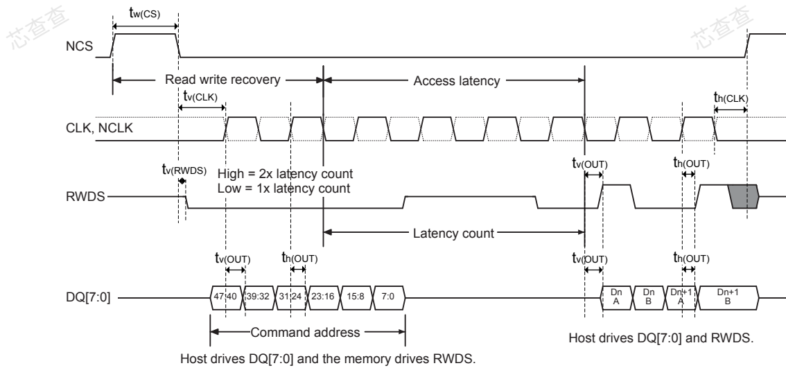
Figure 53. OctoSPI Hyperbus write
