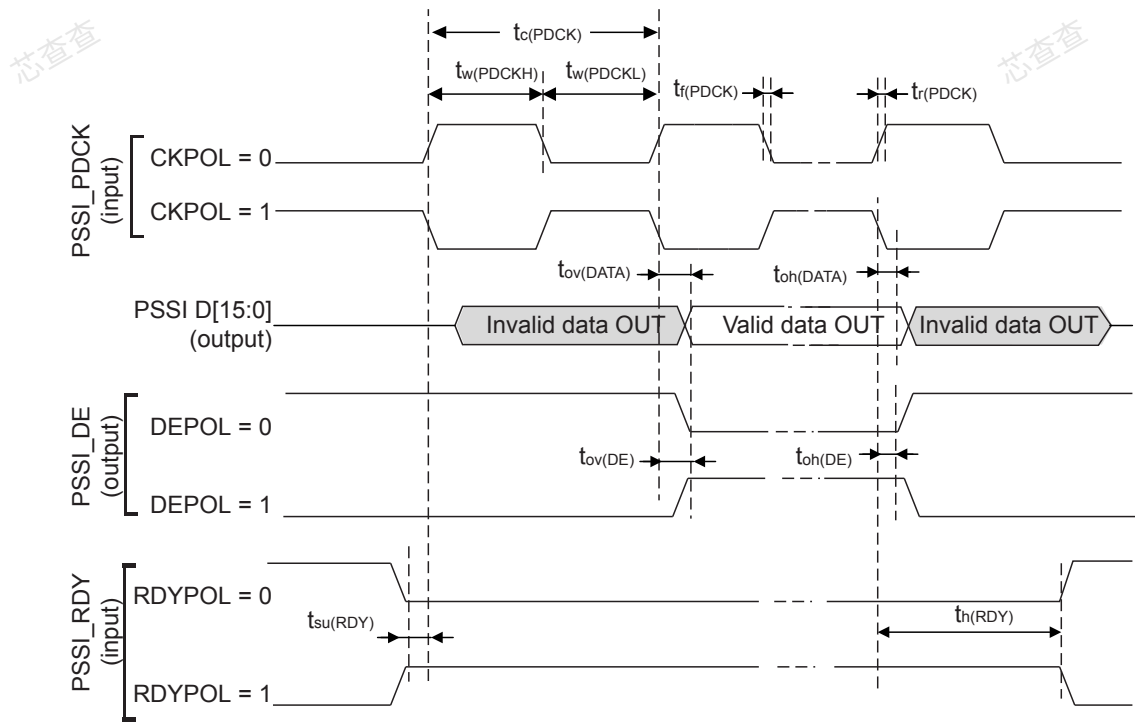
Figure 62. PSSI timing diagram in Transmit mode
