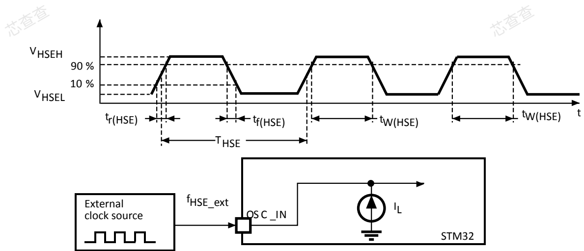
Figure 30. High-speed external clock source AC timing diagram
