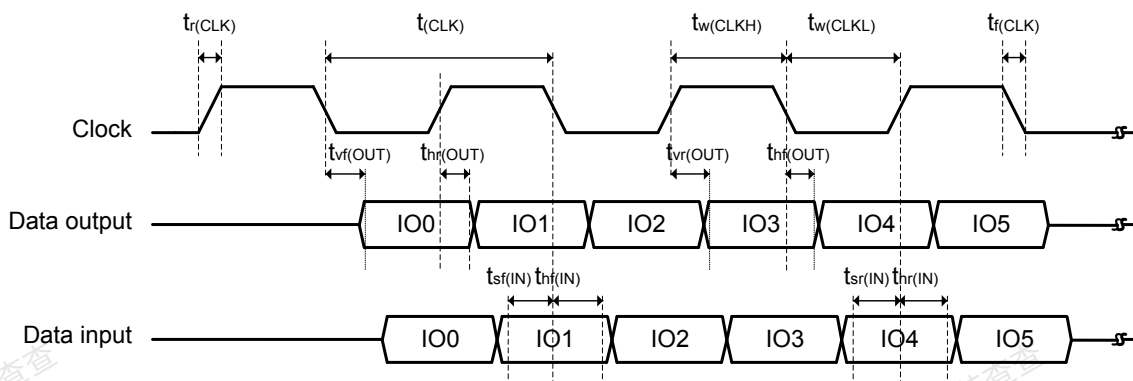
Figure 78. DDR mode
