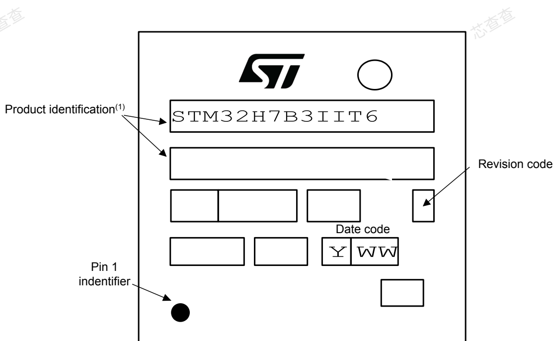
Figure 99. LQFP176 marking example (package top view)
