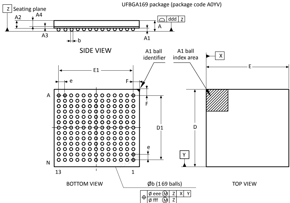
Figure 106. UFBGA169 - Outline
