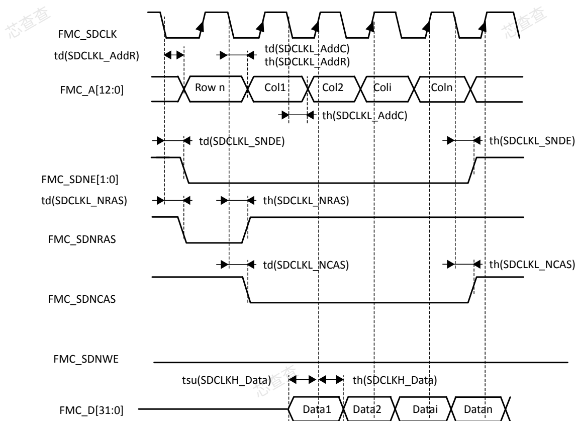
Figure 47. SDRAM read access waveforms (CL = 1)
