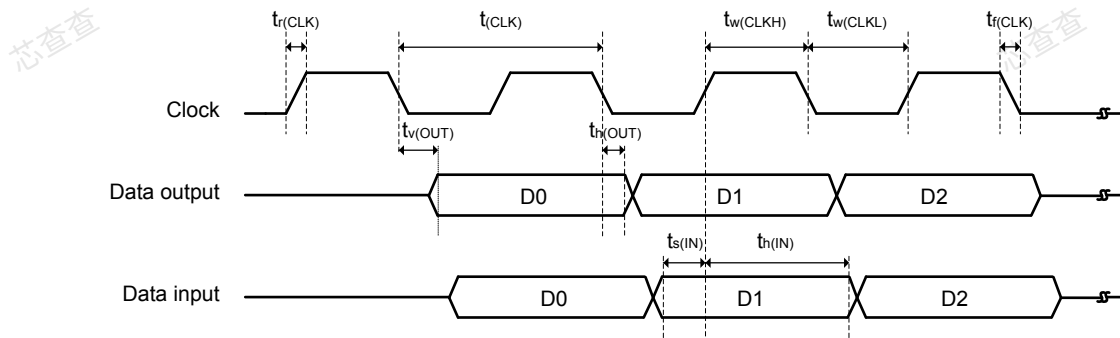
Figure 49. OctoSPI timing diagram - SDR mode
